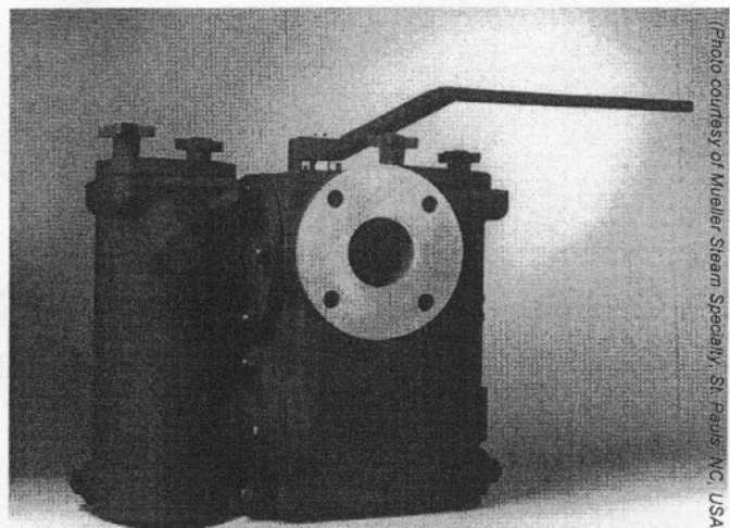
Figure 6 Duplex Strainer
