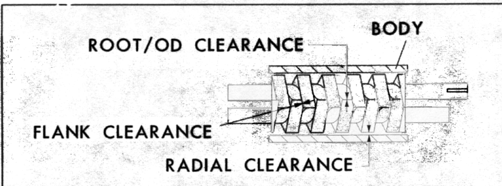
Figure 1 Rotary Pump Running Clearances
