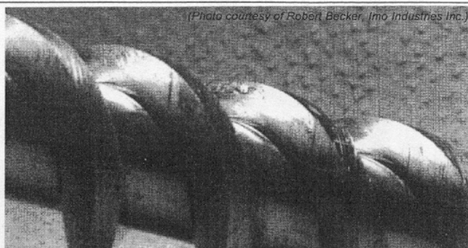
Figure 9 Pump Rotor Damage Caused By Hard Contaminant
