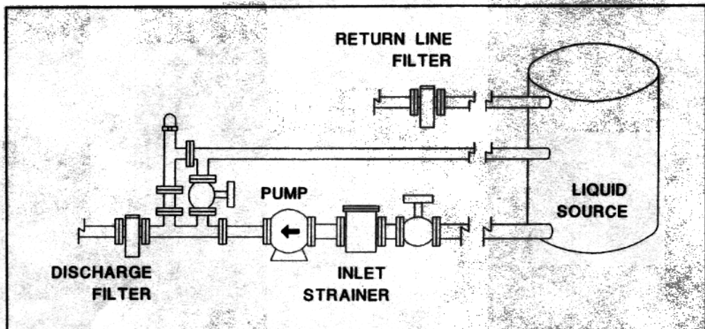
Figure 2 Pump System Strainer and Filters
